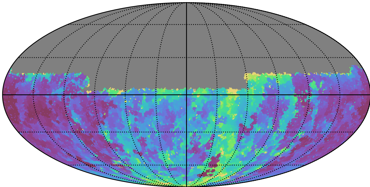
noroll_v3.4_10yrs Yr 1 u band: Min seeingGeom
