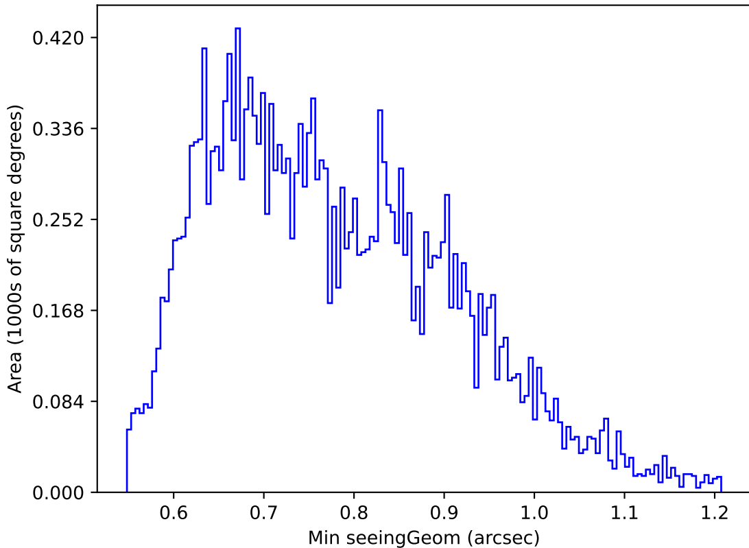
noroll_v3.4_10yrs Yr 1 u band: Min seeingGeom
