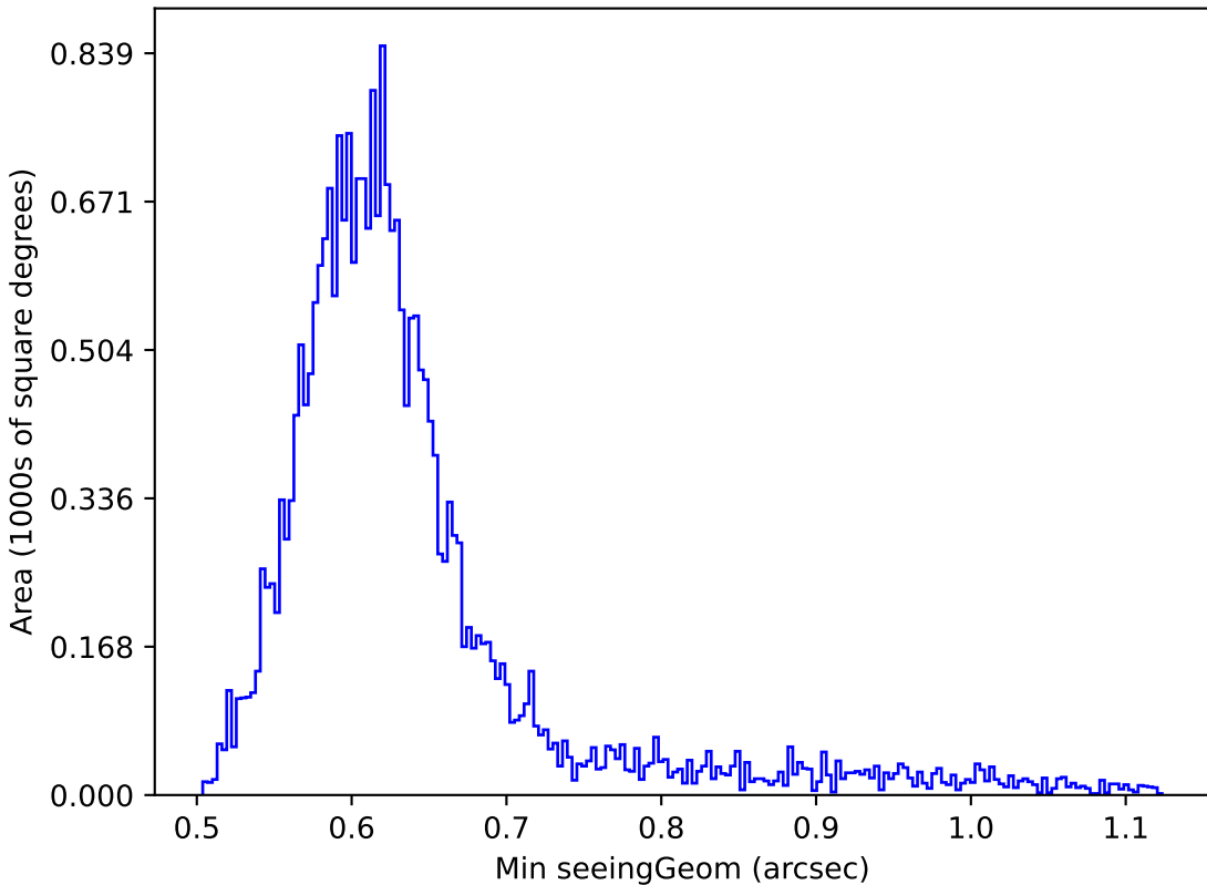
noroll_v3.4_10yrs Yr 1 r band: Min seeingGeom
