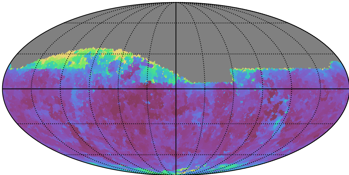
noroll_v3.4_10yrs Yr 1 i band: Min seeingGeom
