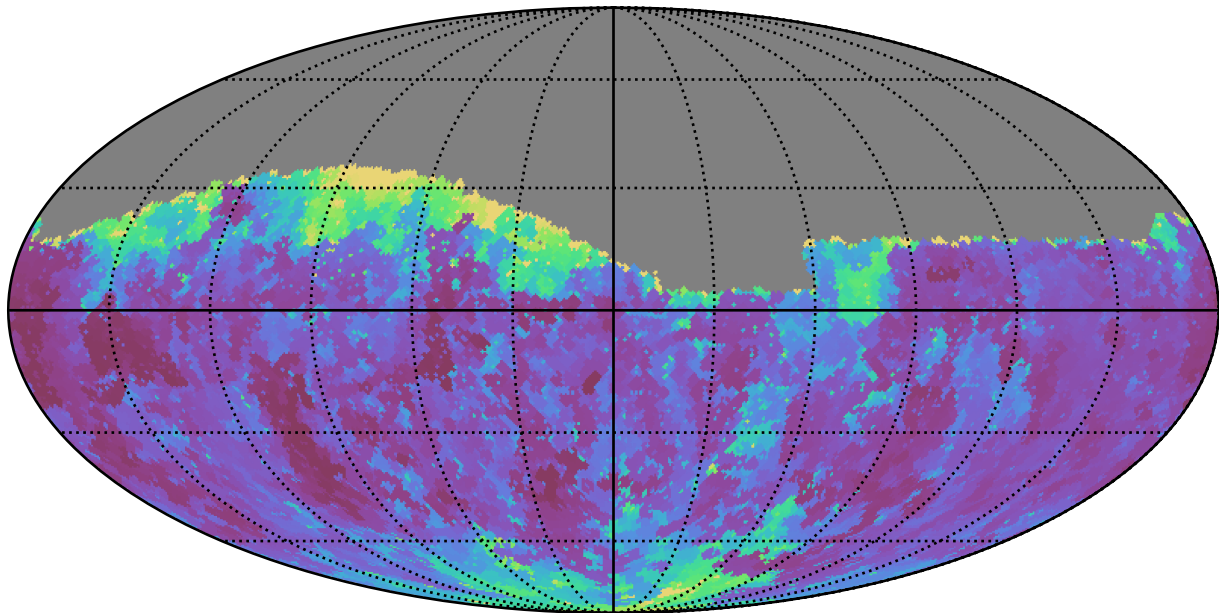
noroll_v3.4_10yrs Yr 1 g band: Min seeingGeom
