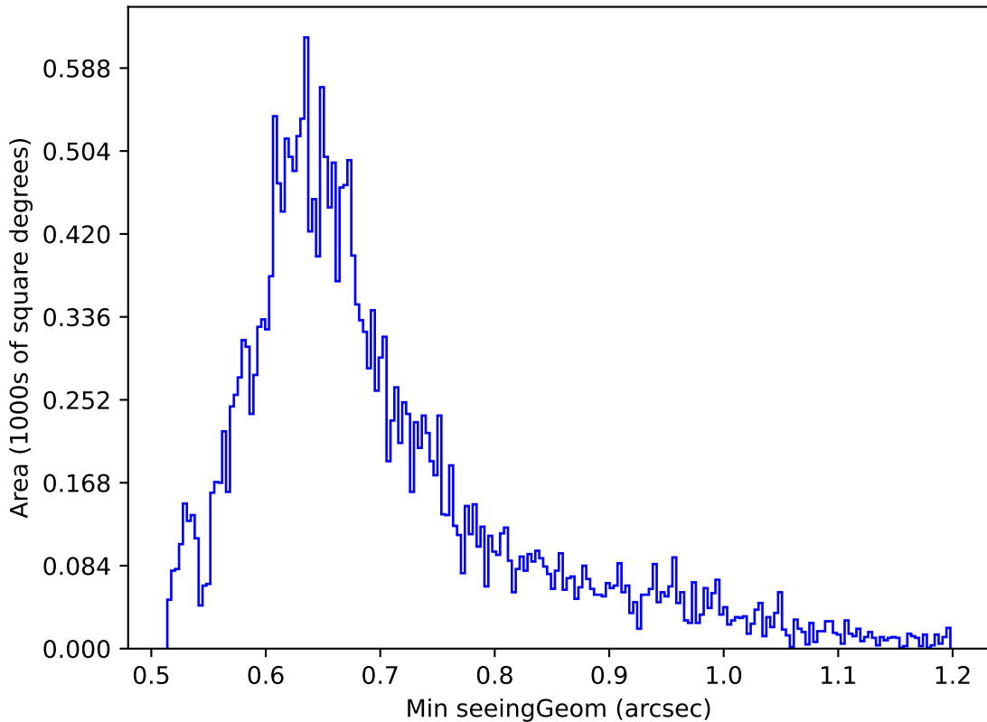
noroll_v3.4_10yrs Yr 1 g band: Min seeingGeom
