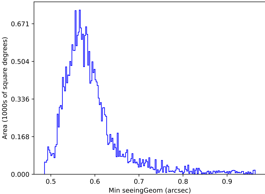
noroll_v3.4_10yrs Yr 1 all bands: Min seeingGeom
