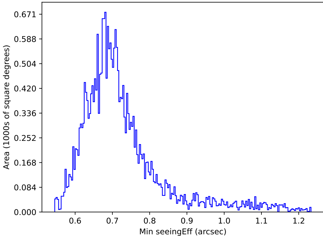
noroll_v3.4_10yrs Yr 1 z band: Min seeingEff
