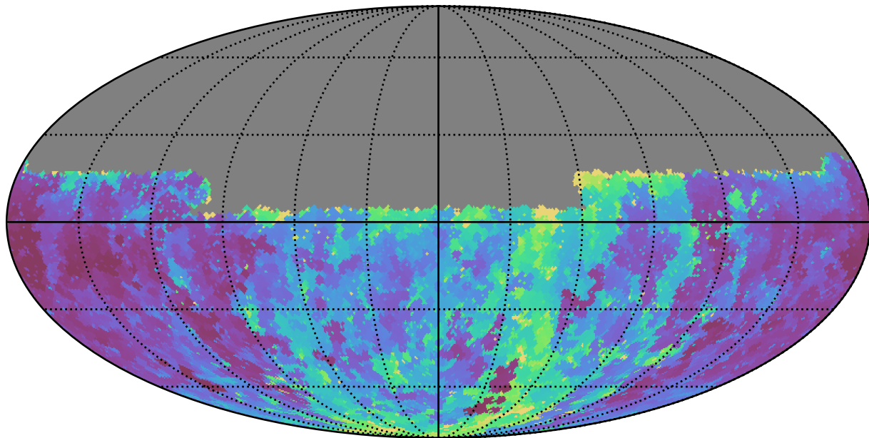
noroll_v3.4_10yrs Yr 1 u band: Min seeingEff
