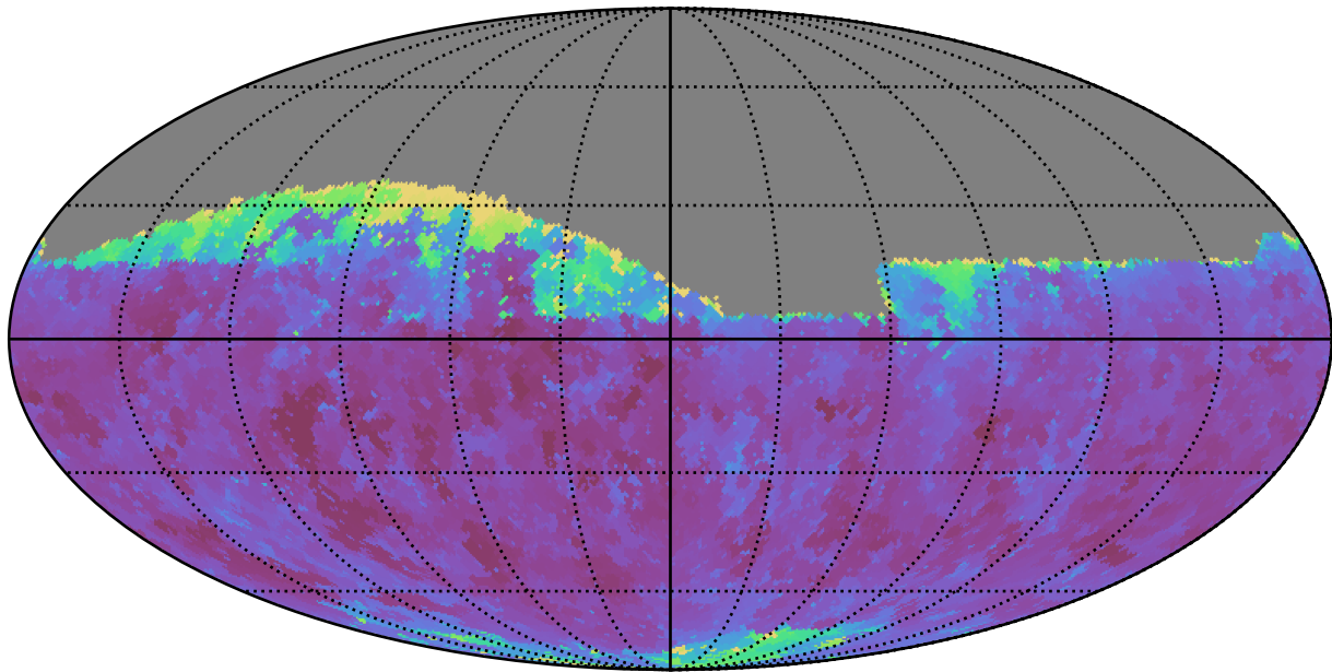
noroll_v3.4_10yrs Yr 1 r band: Min seeingEff
