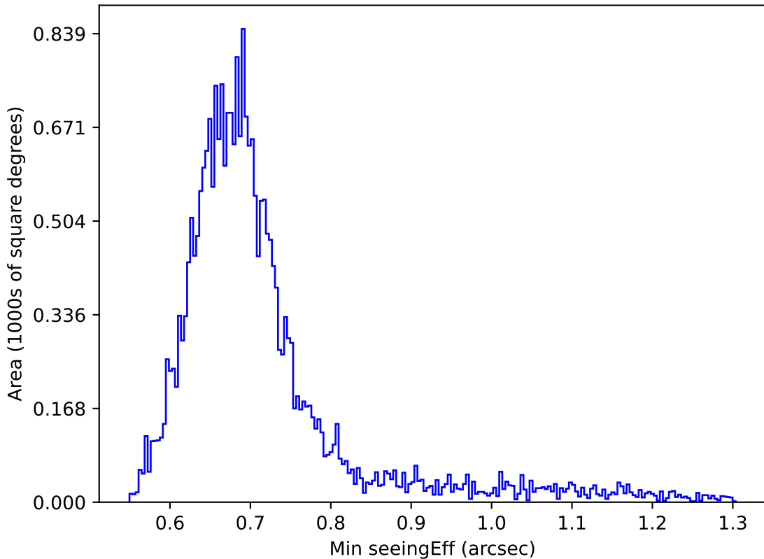
noroll_v3.4_10yrs Yr 1 r band: Min seeingEff
