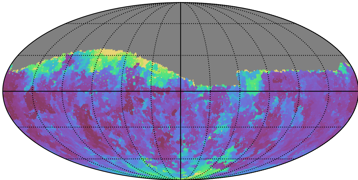
noroll_v3.4_10yrs Yr 1 g band: Min seeingEff
