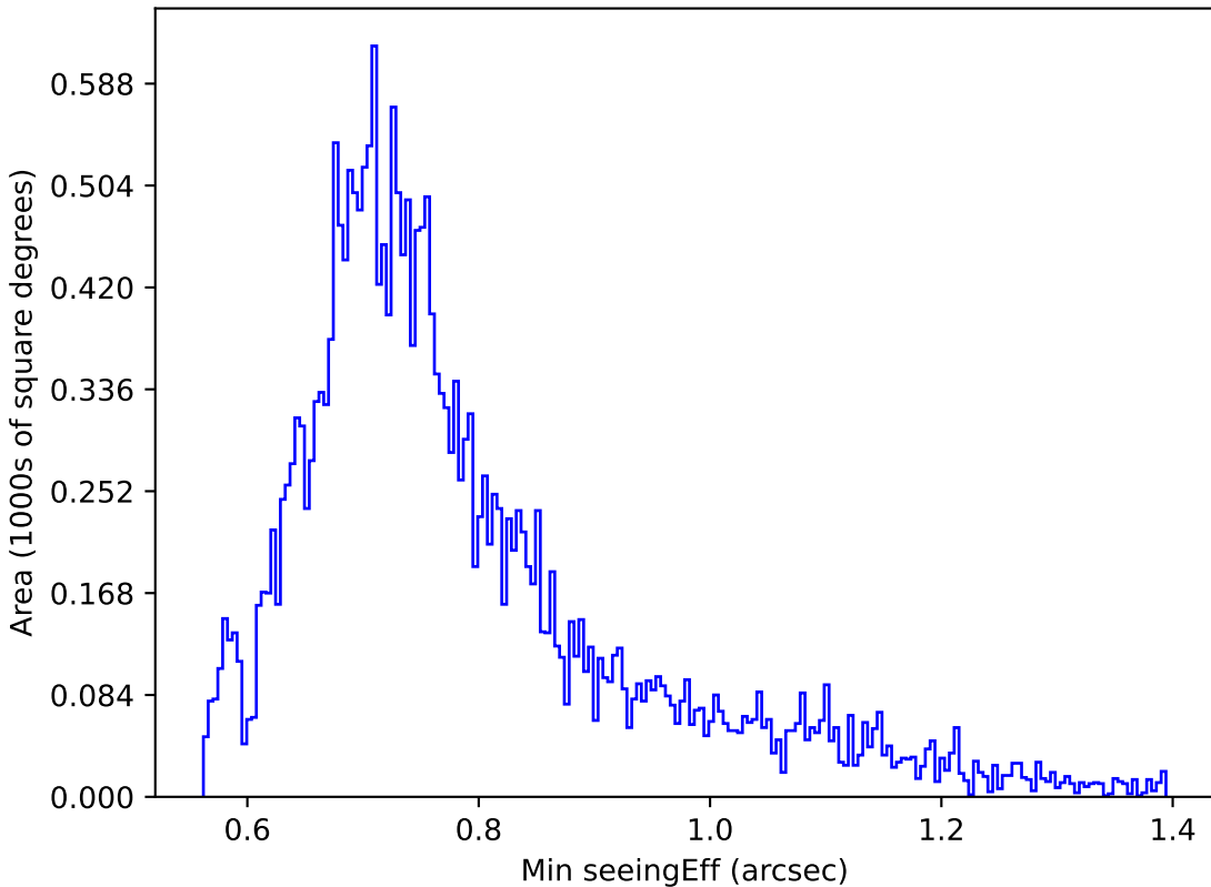
noroll_v3.4_10yrs Yr 1 g band: Min seeingEff
