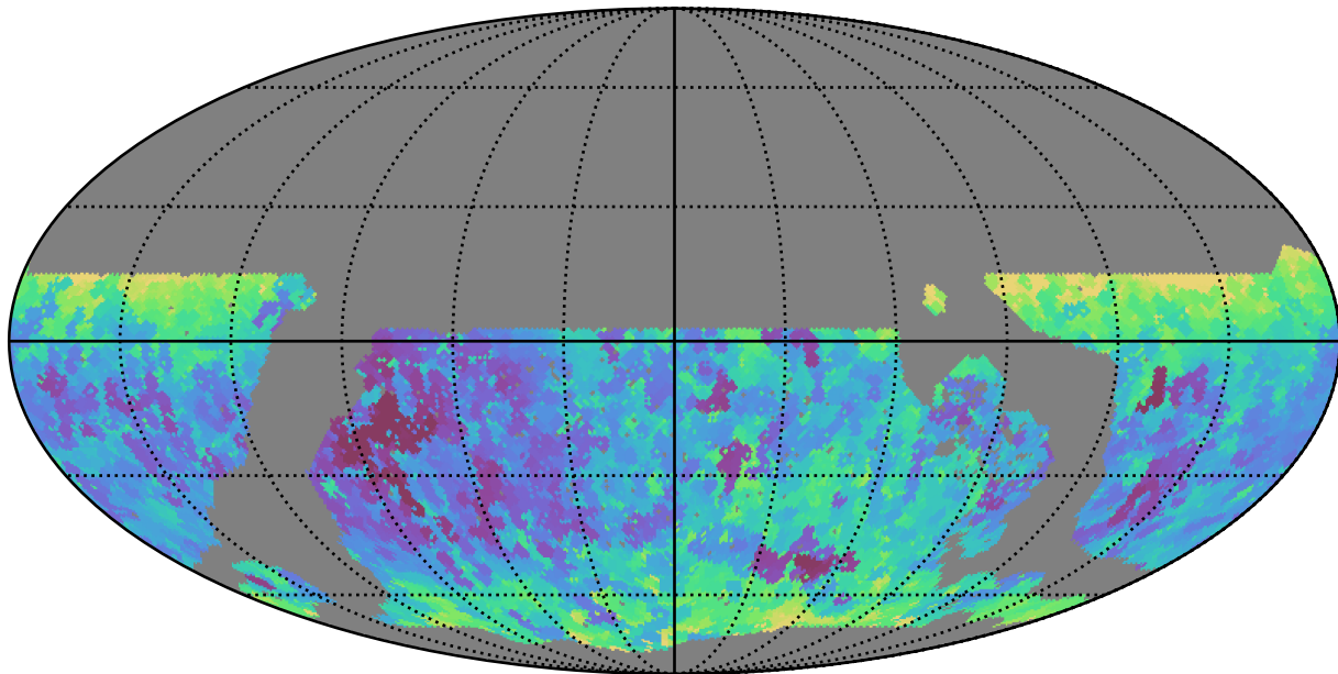
noroll_v3.4_10yrs WFD z band: Min seeingEff
