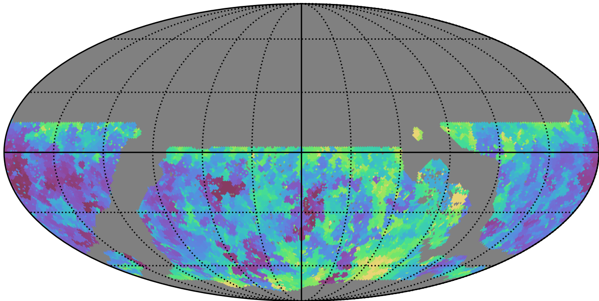
noroll_v3.4_10yrs WFD u band: Min seeingEff
