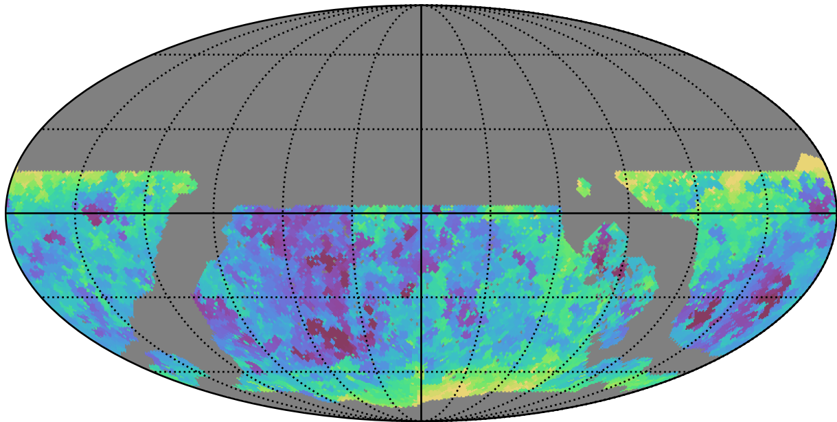
noroll_v3.4_10yrs WFD r band: Min seeingEff
