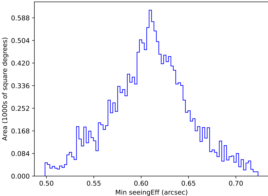
noroll_v3.4_10yrs WFD r band: Min seeingEff
