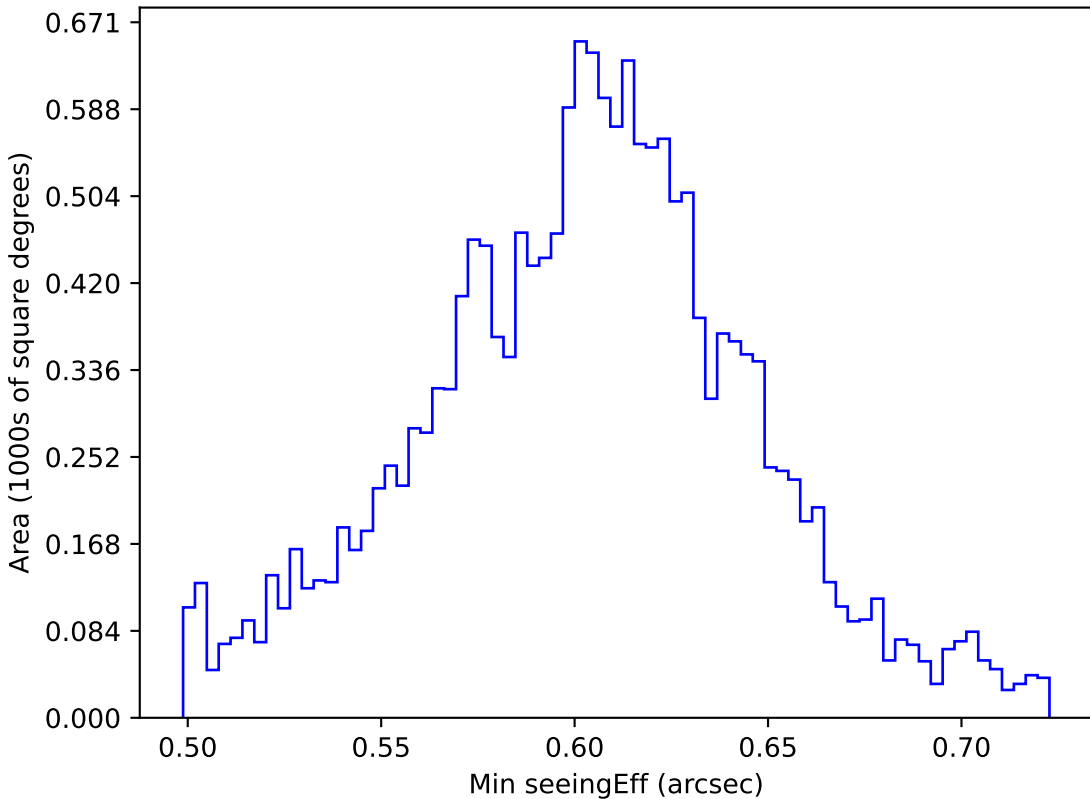
noroll_v3.4_10yrs WFD i band: Min seeingEff
