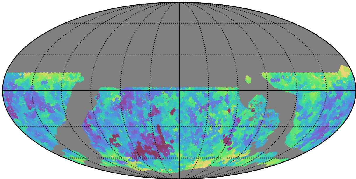
noroll_v3.4_10yrs WFD g band: Min seeingEff
