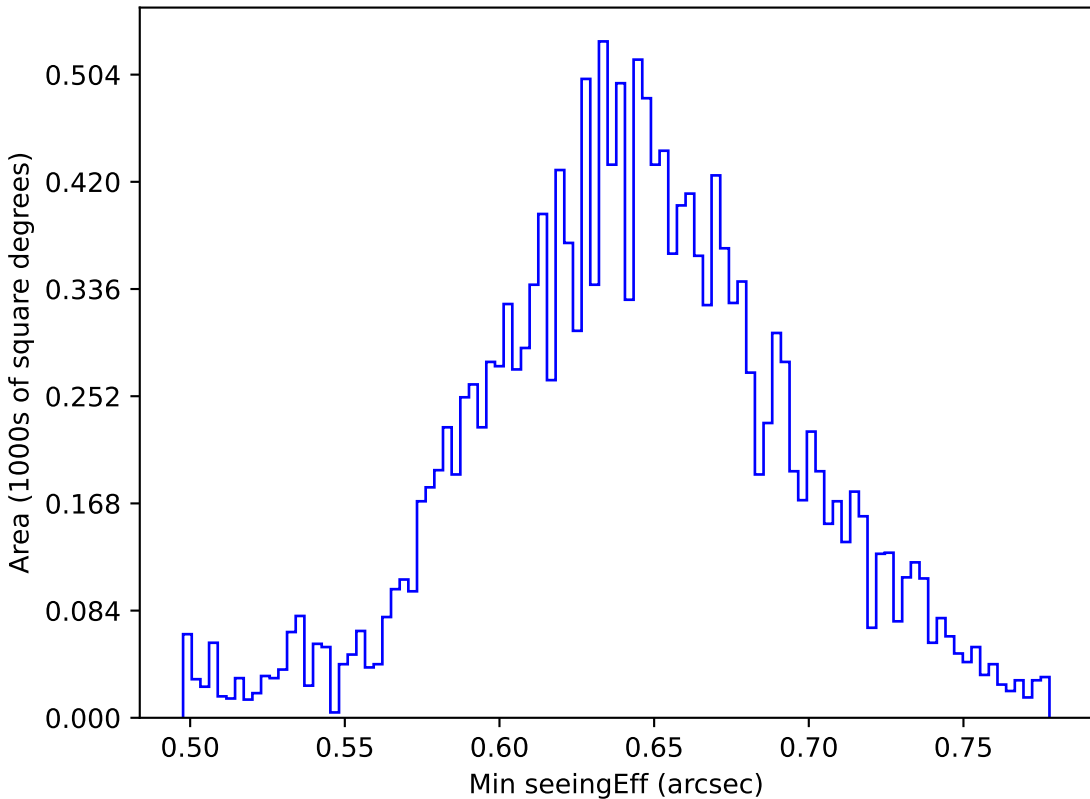
noroll_v3.4_10yrs WFD g band: Min seeingEff
