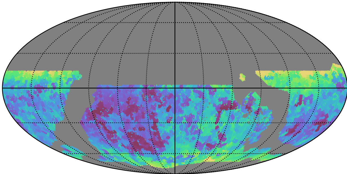
noroll_v3.4_10yrs WFD all bands: Min seeingEff
