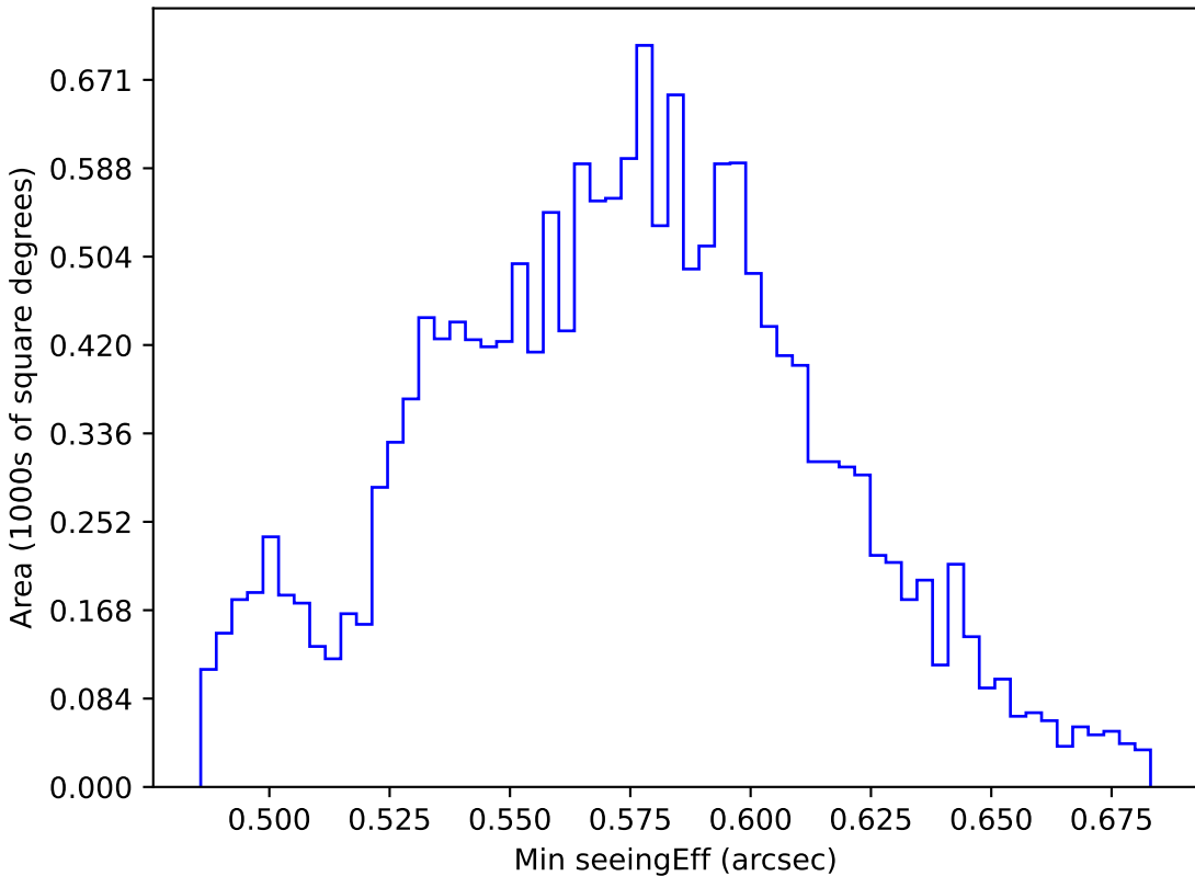
noroll_v3.4_10yrs WFD all bands: Min seeingEff
