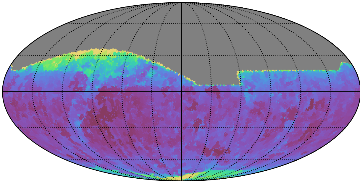
noroll_v3.4_10yrs All sky z band: Min seeingEff
