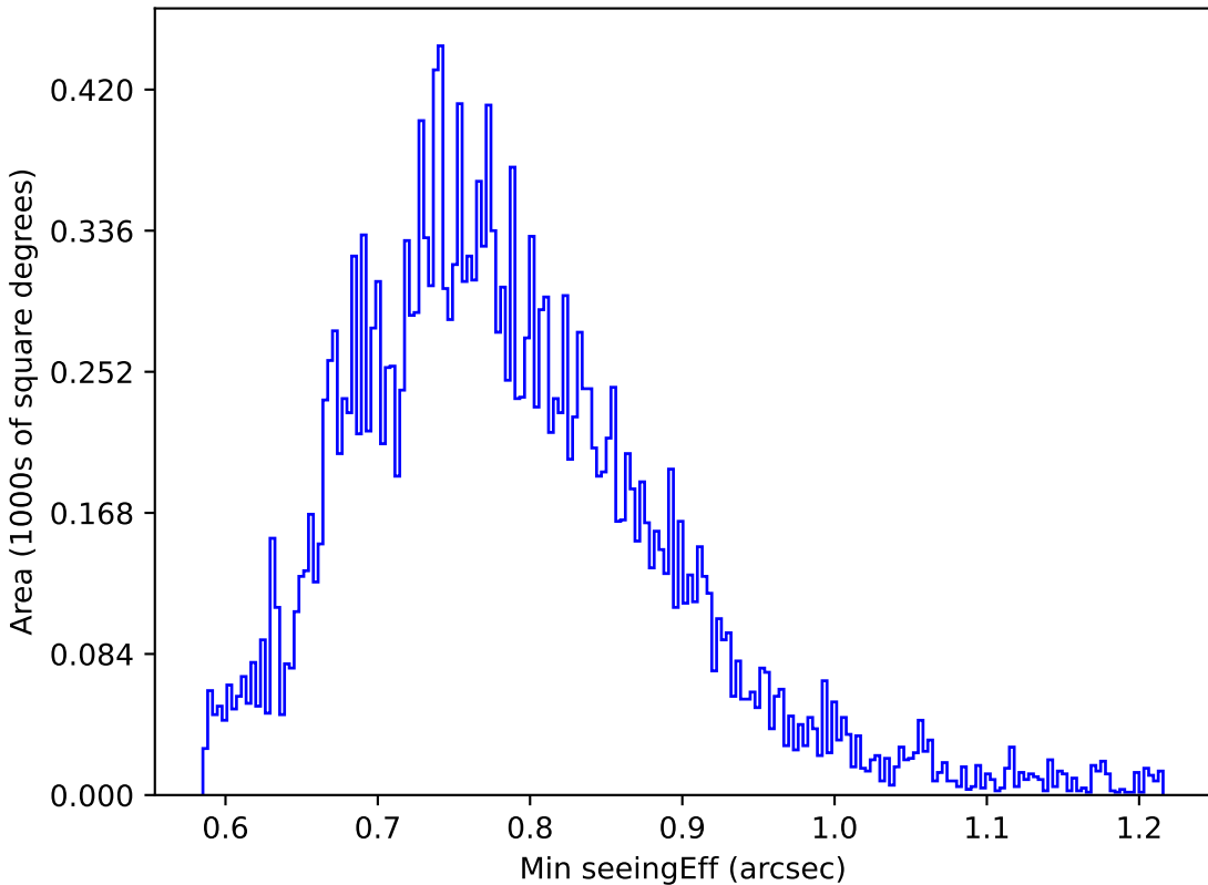
noroll_v3.4_10yrs All sky u band: Min seeingEff
