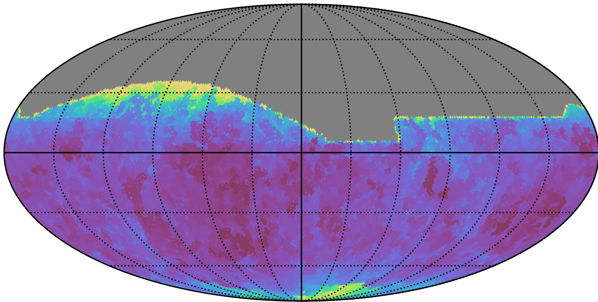
noroll_v3.4_10yrs All sky r band: Min seeingEff
