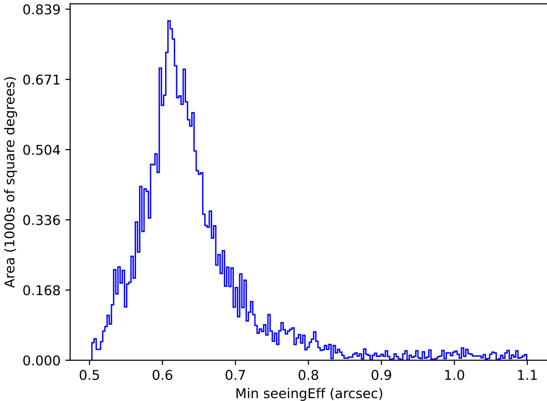
noroll_v3.4_10yrs All sky r band: Min seeingEff
