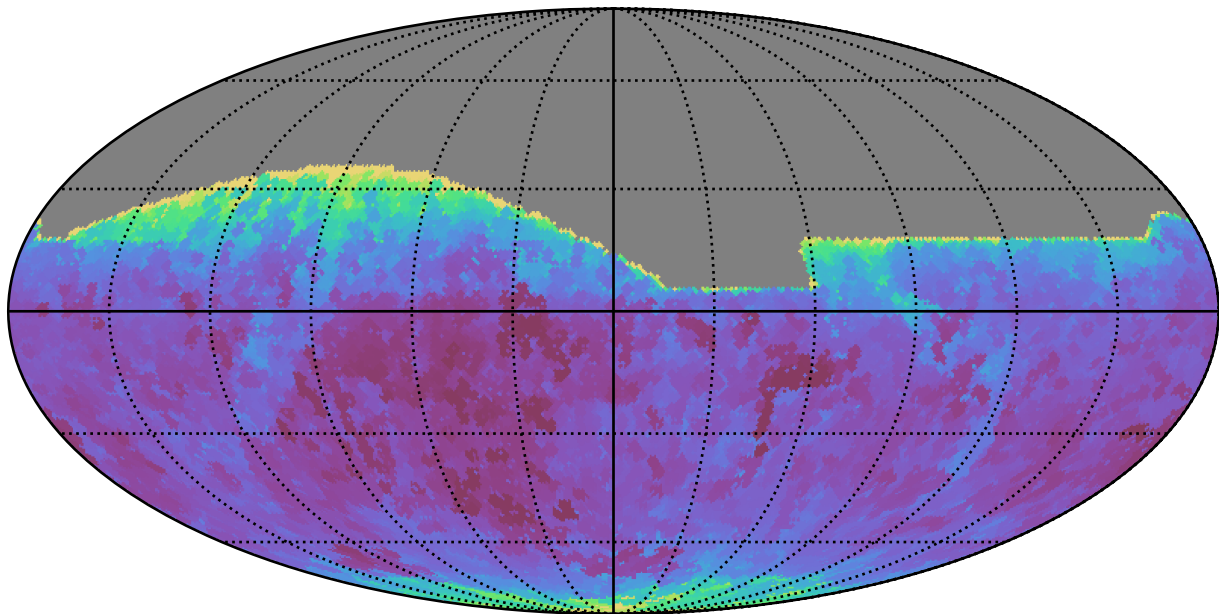
noroll_v3.4_10yrs All sky i band: Min seeingEff
