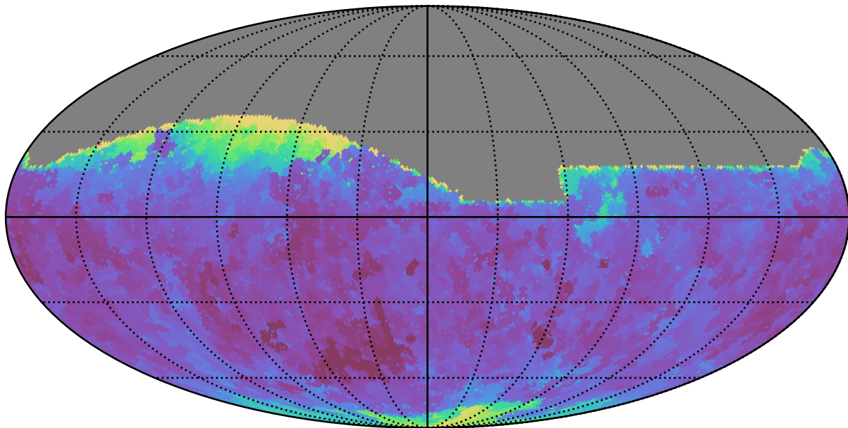
noroll_v3.4_10yrs All sky g band: Min seeingEff
