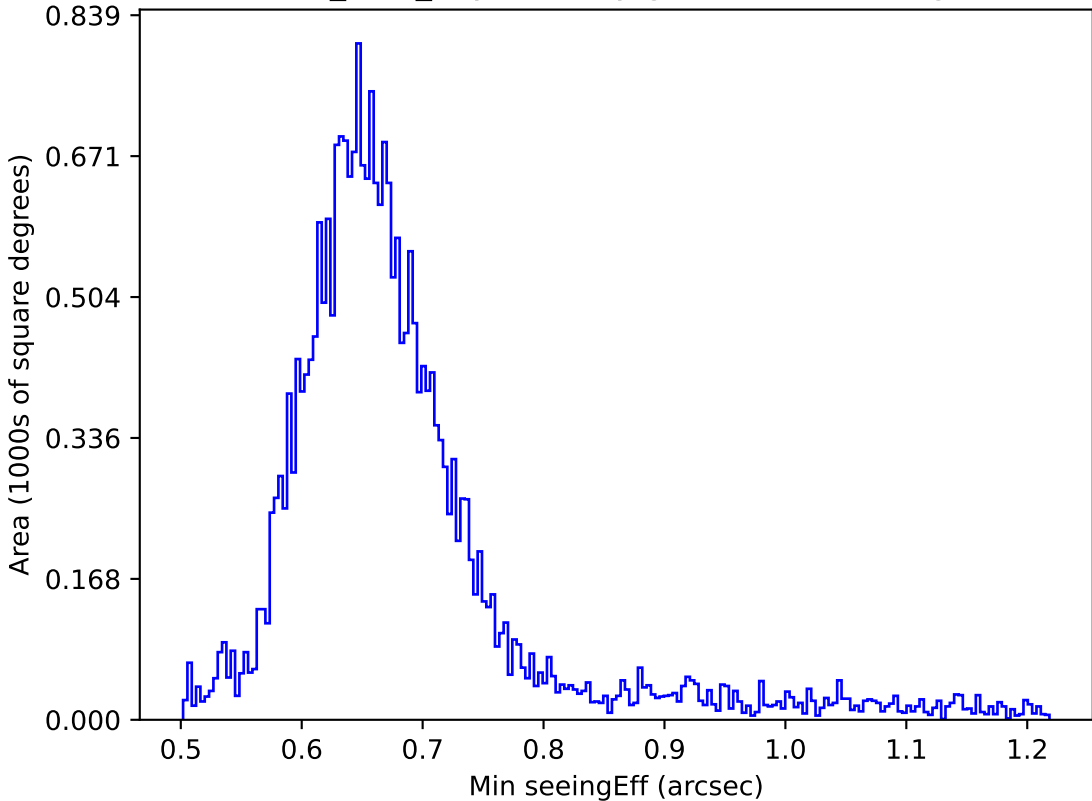
noroll_v3.4_10yrs All sky g band: Min seeingEff
