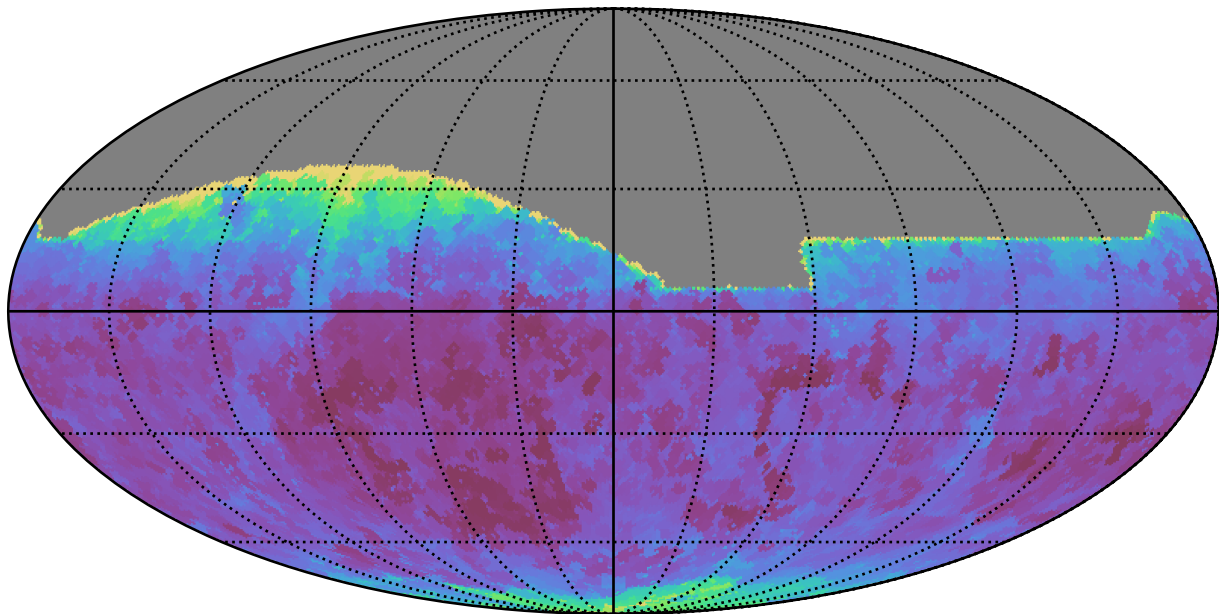
noroll_v3.4_10yrs All sky all bands: Min seeingEff
