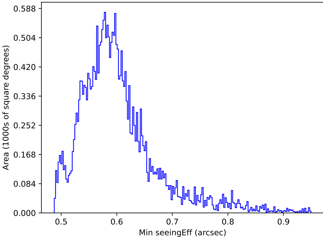
noroll_v3.4_10yrs All sky all bands: Min seeingEff
