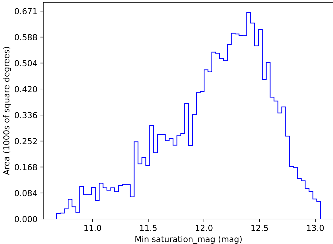
noroll_v3.4_10yrs WFD z band: Min saturation_mag
