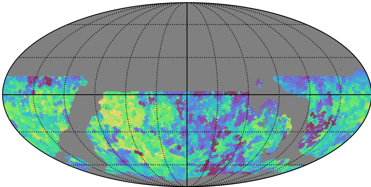
noroll_v3.4_10yrs WFD u band: Min saturation_mag
