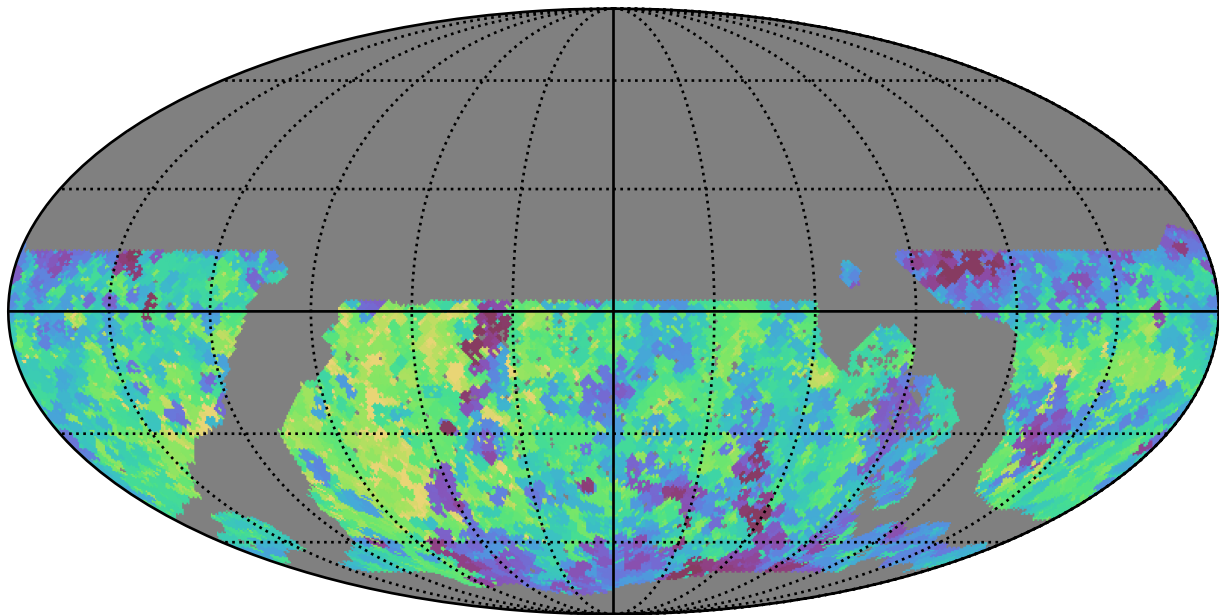
noroll_v3.4_10yrs WFD g band: Min saturation_mag
