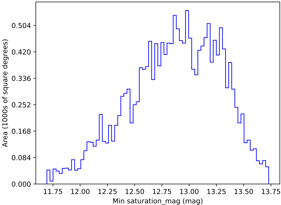
noroll_v3.4_10yrs WFD g band: Min saturation_mag
