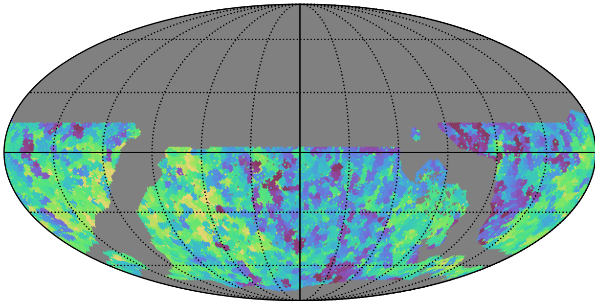
noroll_v3.4_10yrs WFD all bands: Min saturation_mag
