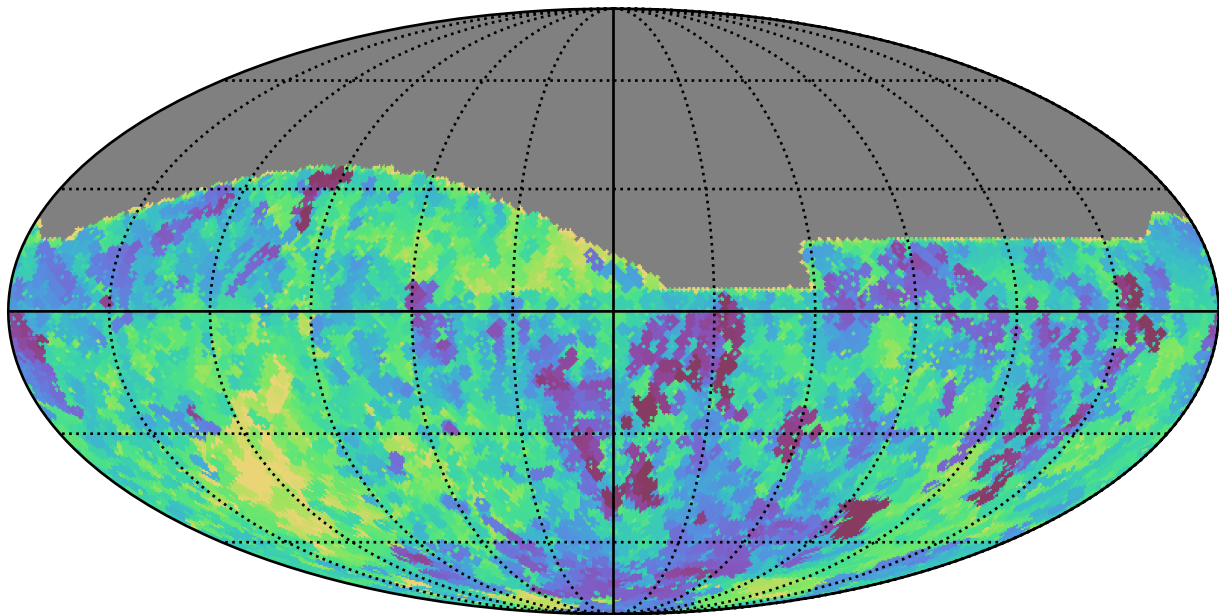
noroll_v3.4_10yrs All sky z band: Min saturation_mag
