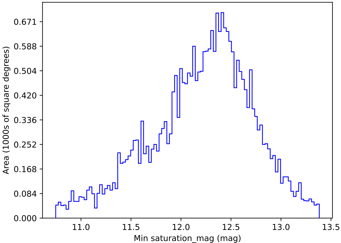
noroll_v3.4_10yrs All sky z band: Min saturation_mag
