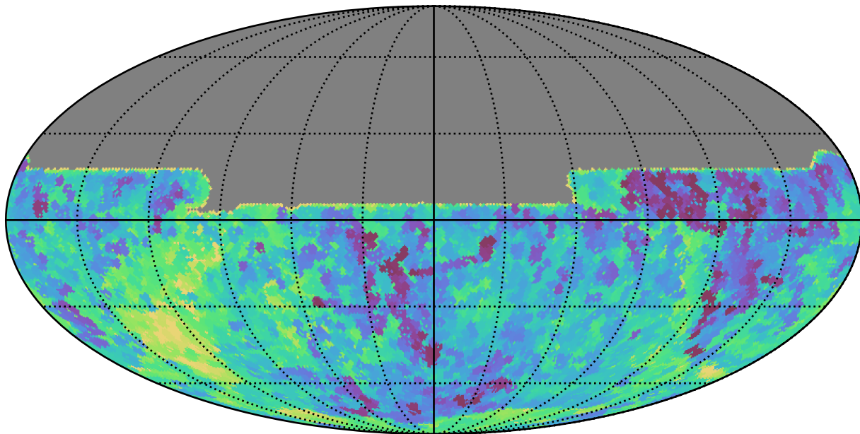
noroll_v3.4_10yrs All sky y band: Min saturation_mag
