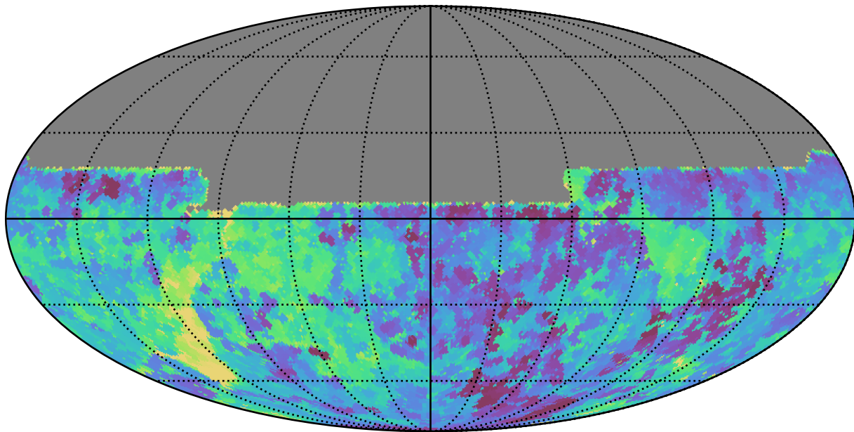
noroll_v3.4_10yrs All sky u band: Min saturation_mag
