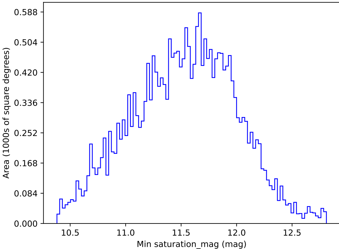
noroll_v3.4_10yrs All sky u band: Min saturation_mag
