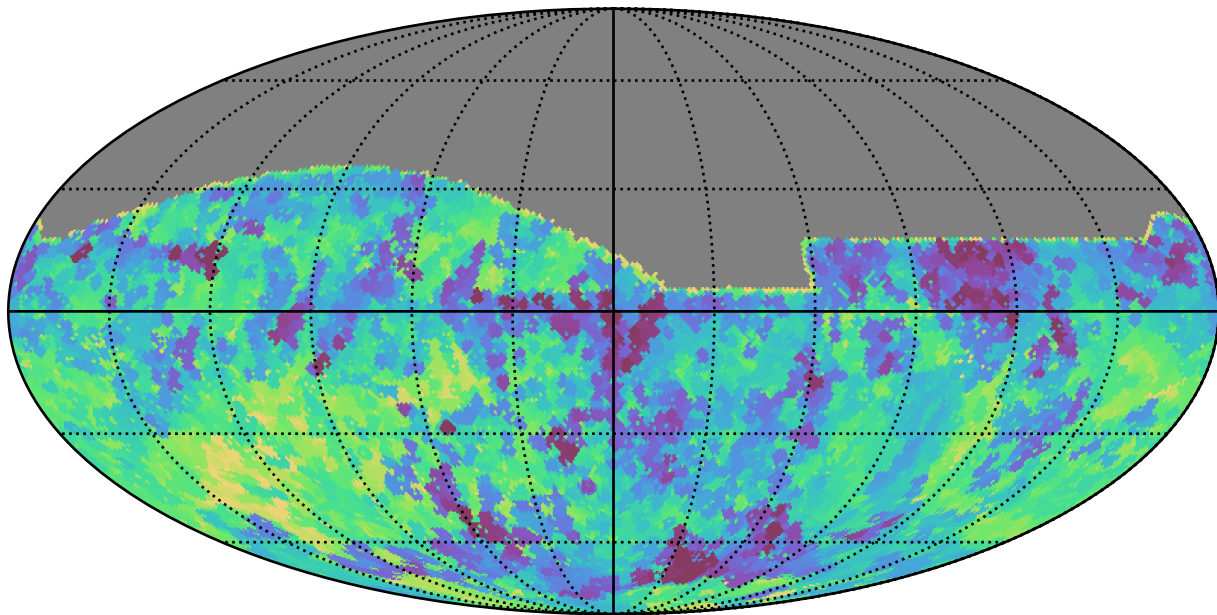
noroll_v3.4_10yrs All sky r band: Min saturation_mag
