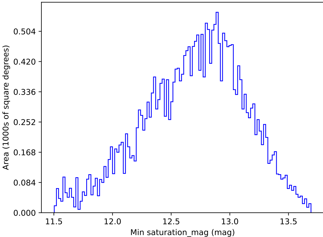
noroll_v3.4_10yrs All sky r band: Min saturation_mag
