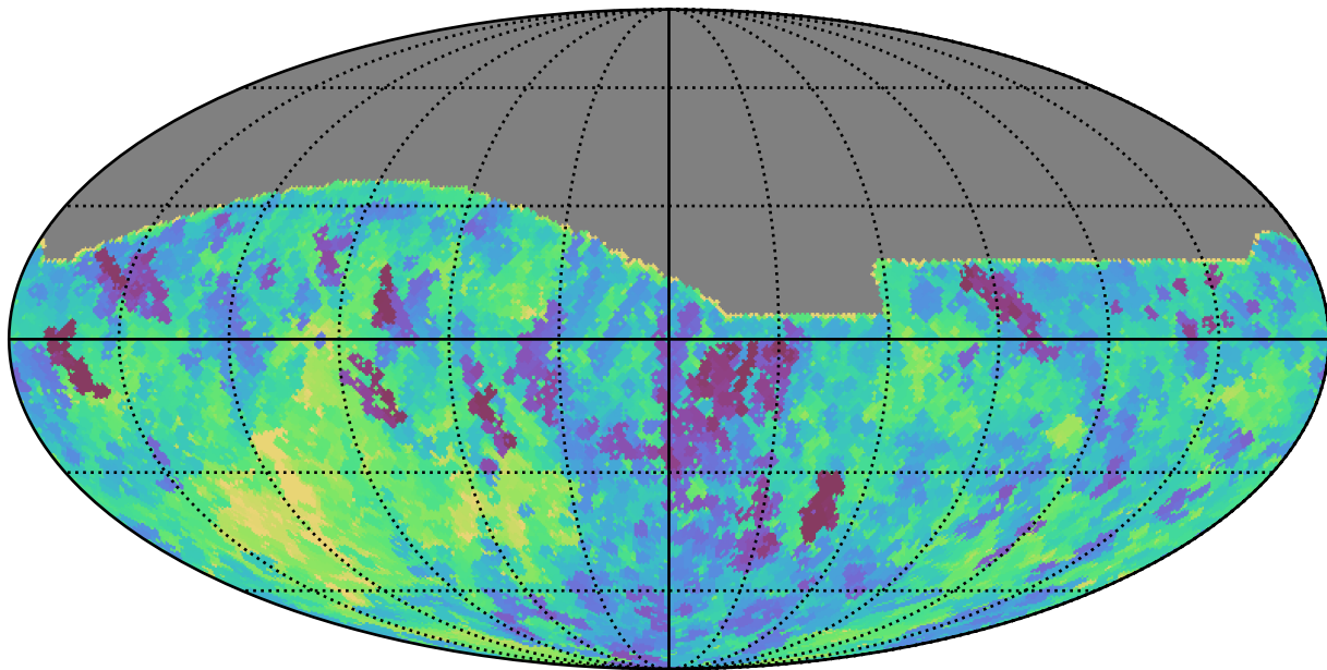
noroll_v3.4_10yrs All sky i band: Min saturation_mag
