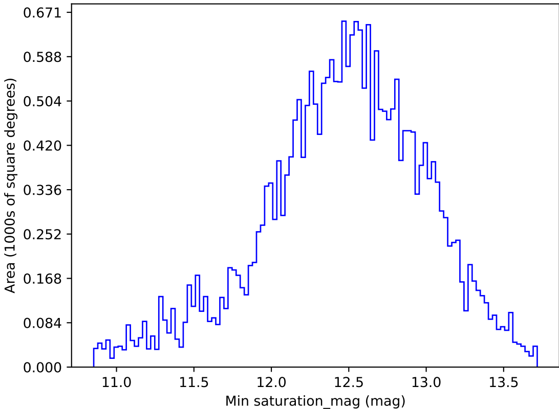
noroll_v3.4_10yrs All sky i band: Min saturation_mag
