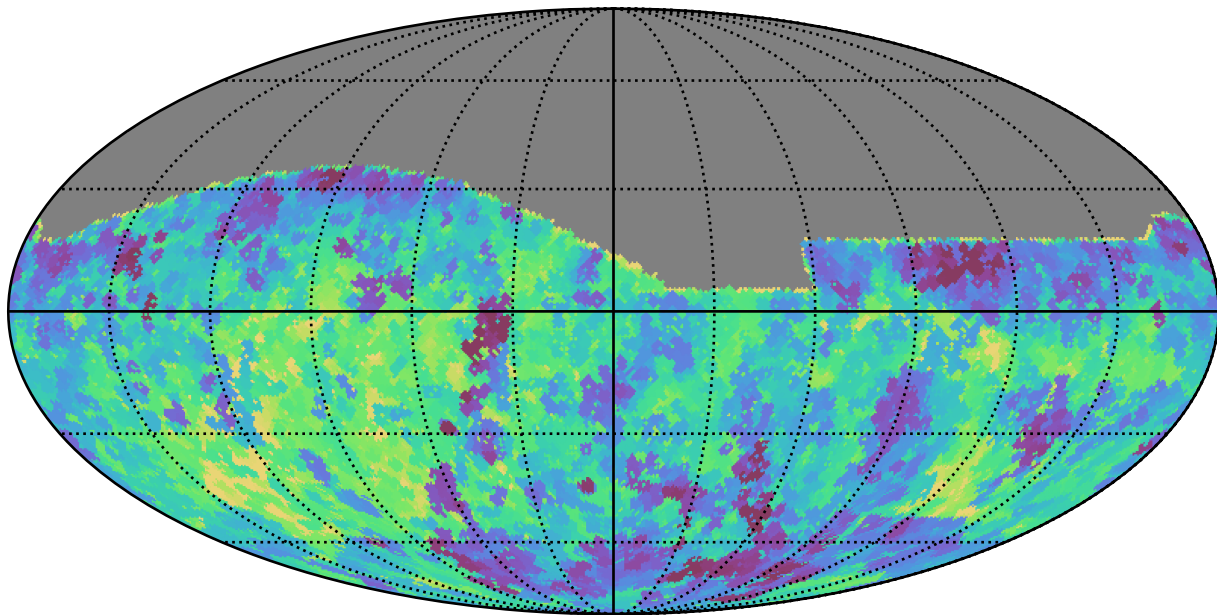
noroll_v3.4_10yrs All sky g band: Min saturation_mag
