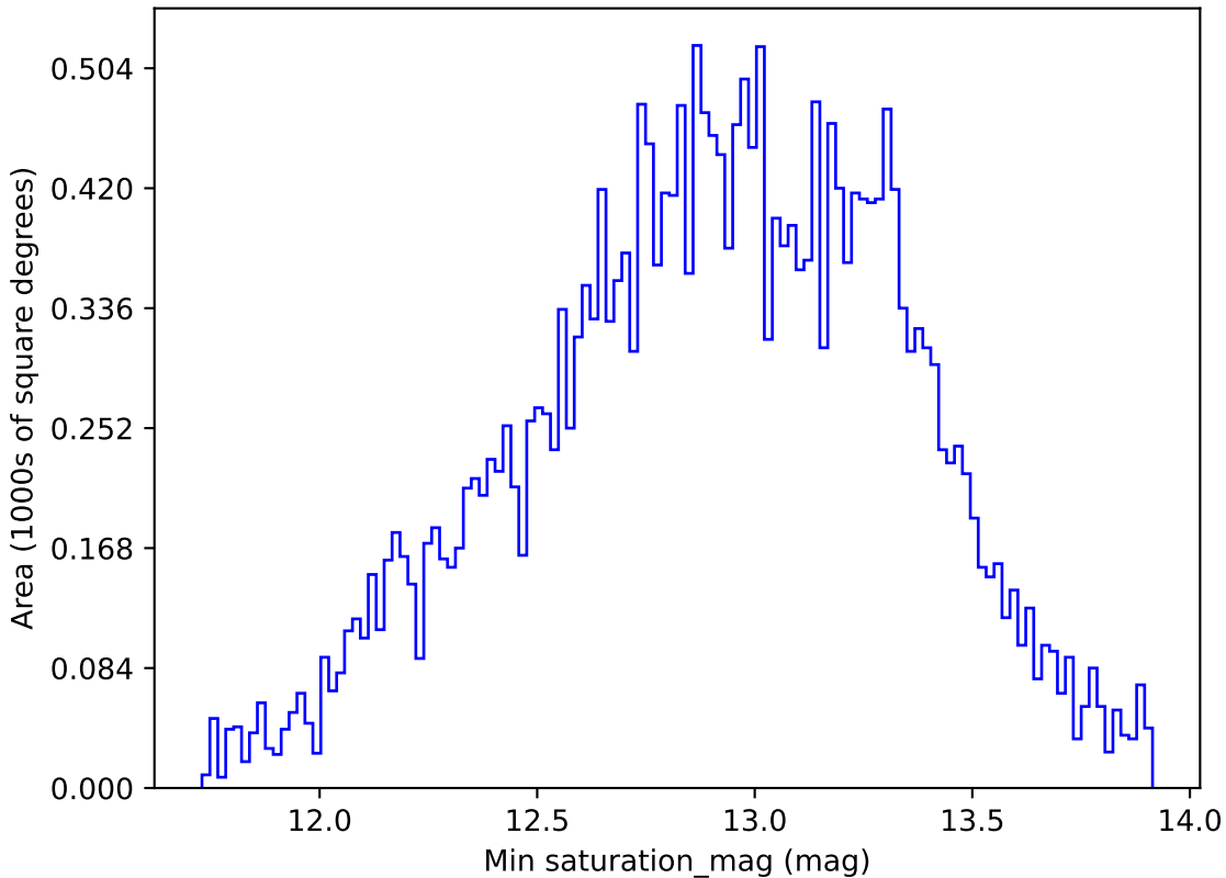
noroll_v3.4_10yrs All sky g band: Min saturation_mag
