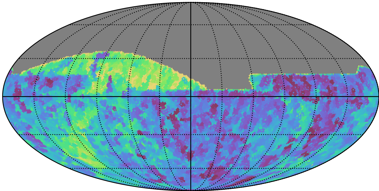
noroll_v3.4_10yrs All sky all bands: Min saturation_mag
