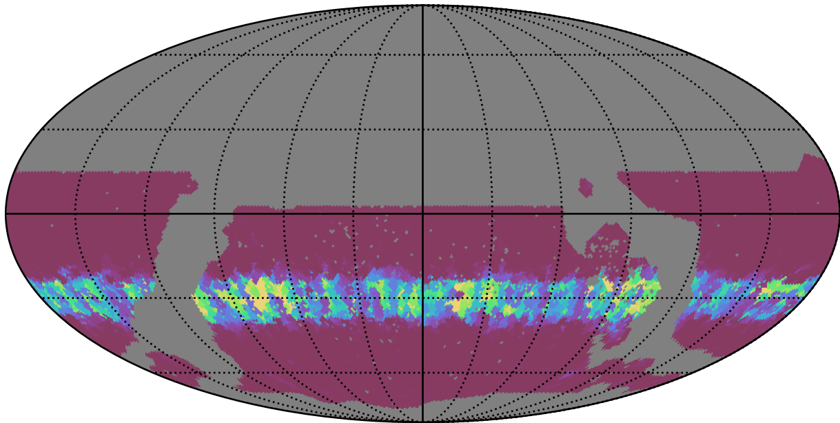
noroll_v3.4_10yrs WFD u band: Min normairmass
