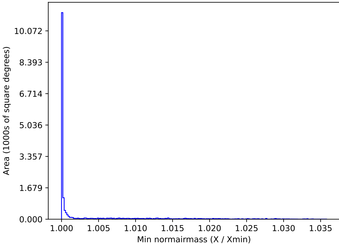
noroll_v3.4_10yrs WFD u band: Min normairmass
